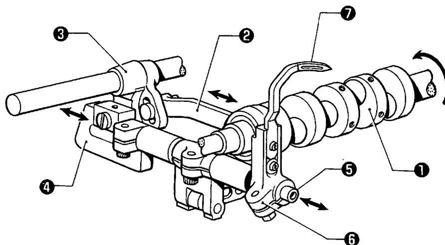
[Longitudinal feed mechanism]
