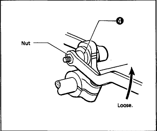
(2) Loosen the nut, and change the position of the main feed shaft ❹.
